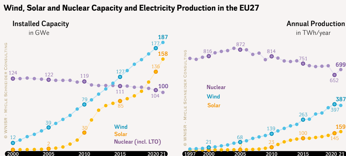
Figure 61 · Wind, Solar and Nuclear Capacity and Electricity Production in the EU27 (Absolute Numbers)
