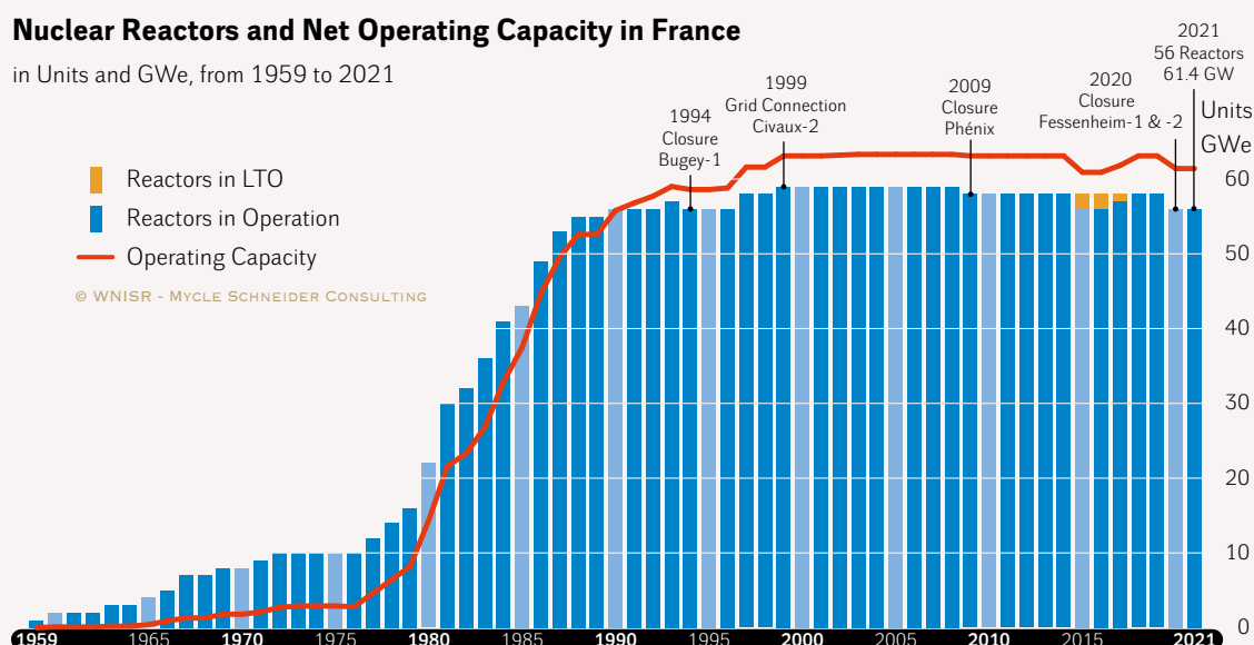
Figure 23 · Operating Fleet and Capacity in France
