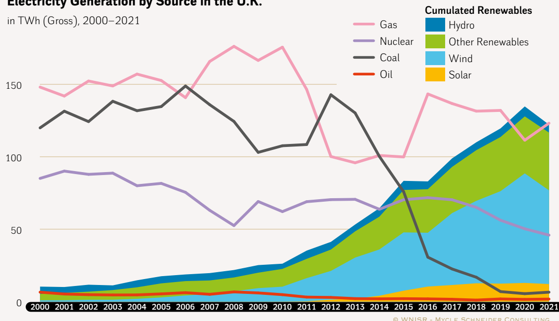
Figure 38 · Electricity Generation by Source in the U.K. 2000–2021
