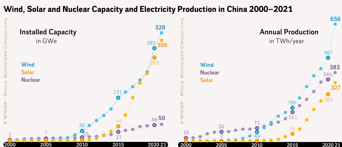
Figure 58 · Wind, Solar and Nuclear Installed Capacity and Electricity Production in China, 2000–2021
