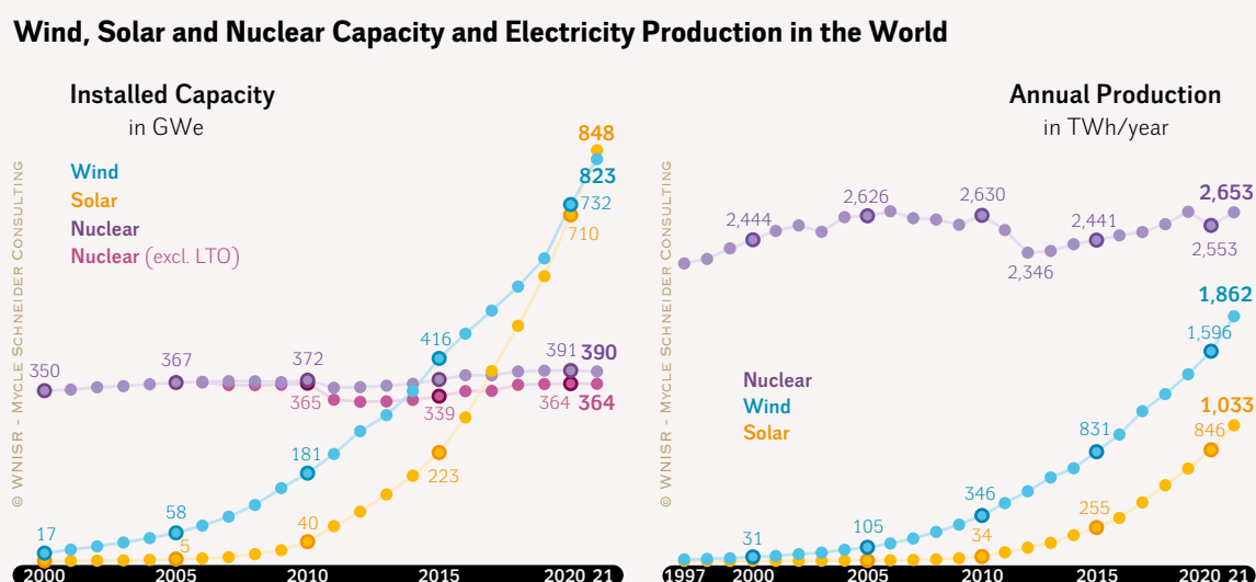
Figure 56 · Wind, Solar and Nuclear Installed Capacity and Electricity Production in the World
