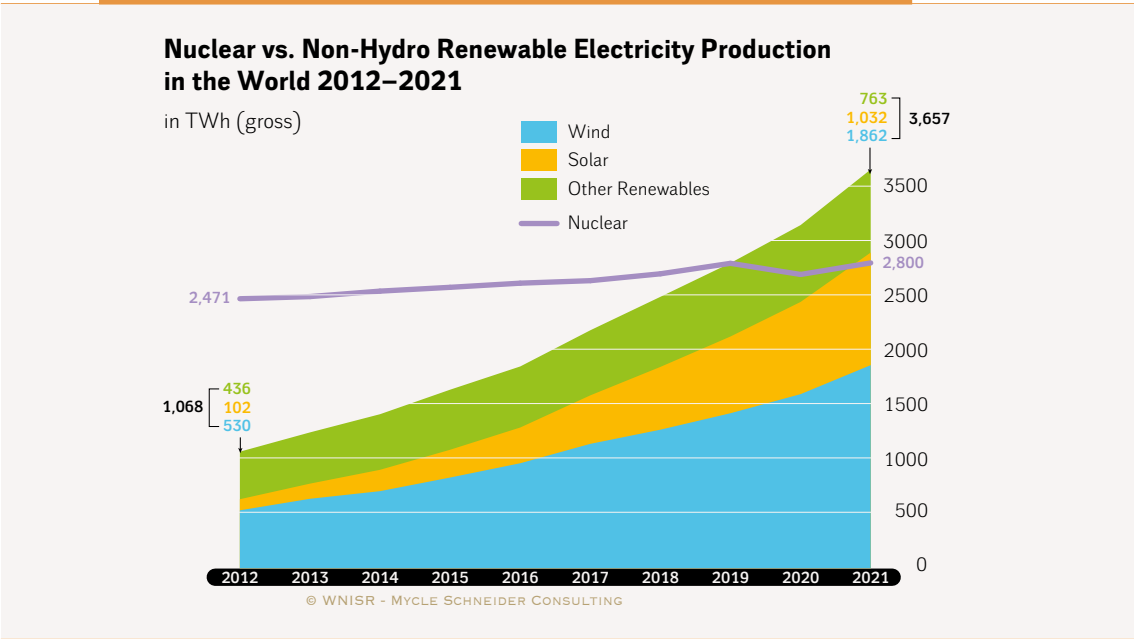
Figure 55 · Nuclear vs. Non-Hydro Renewable Electricity Production in the World
