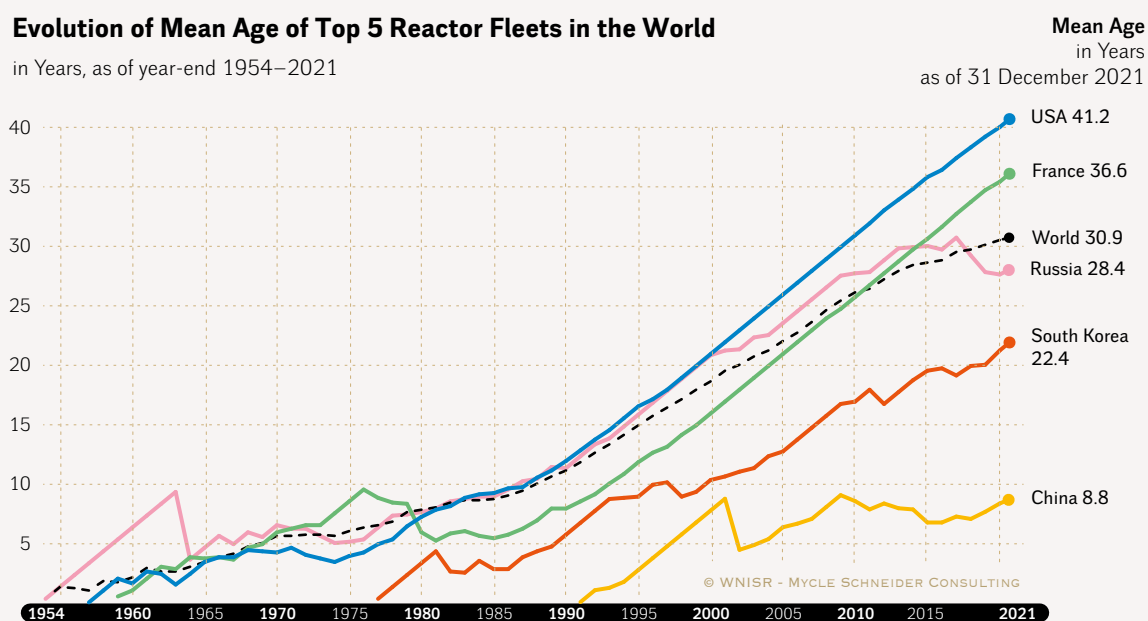
Figure 16 · Reactor-Fleet Age of Top 5 Nuclear Generators
